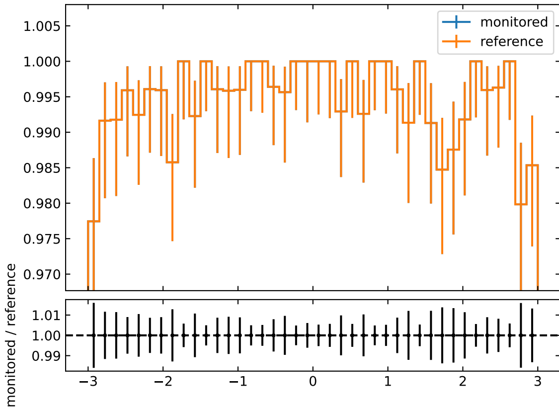
Tracking efficiency with p_T > 1 \text{ GeV/c}
