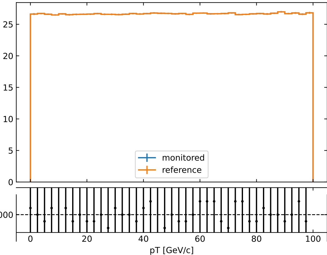
Number of total states vs. pT
