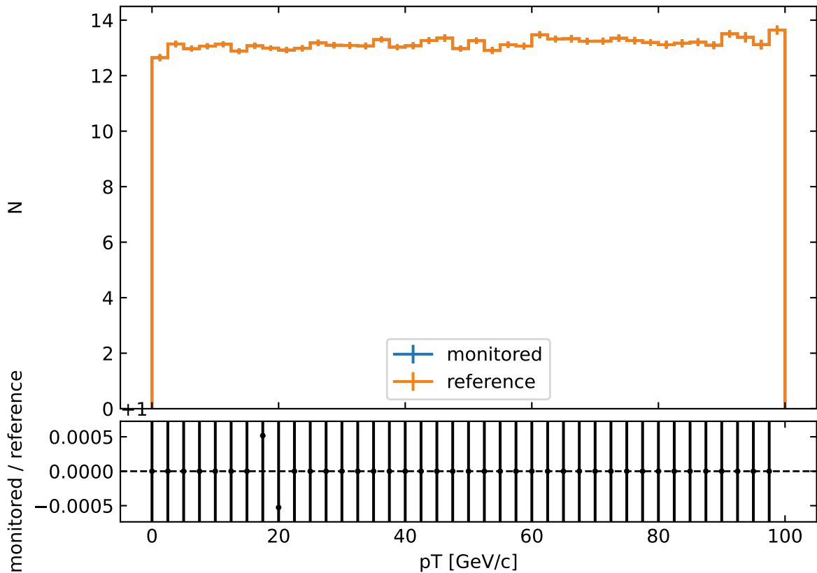
Number of measurements vs. pT
