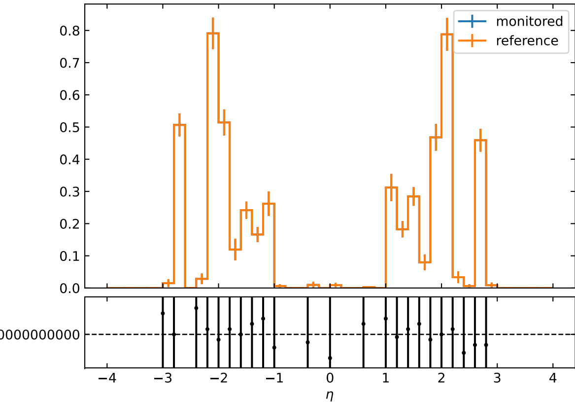
Number of outliers vs. \eta
