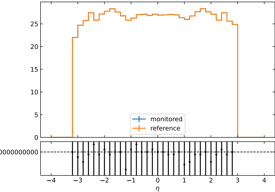
Number of total states vs. \eta
