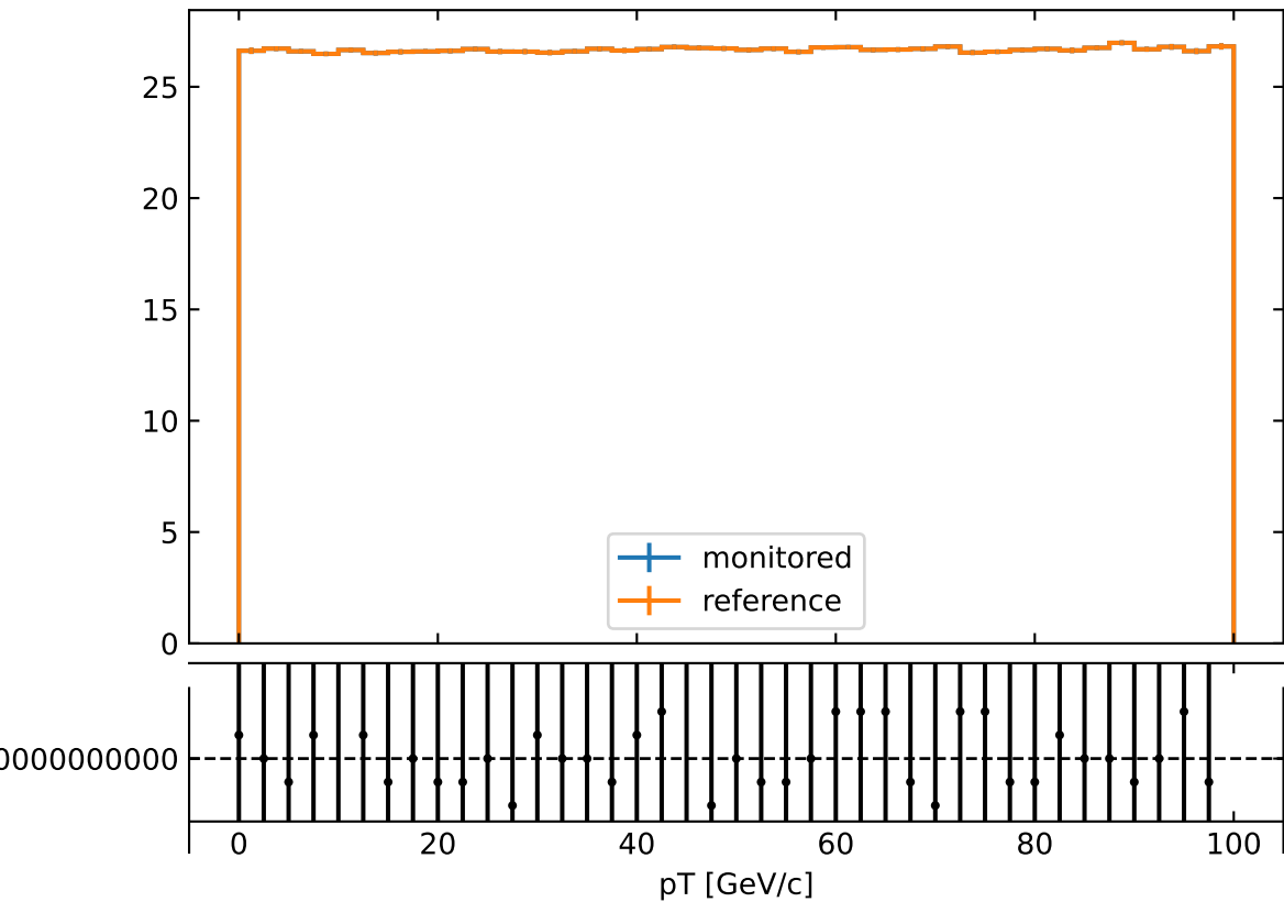
Number of total states vs. pT
