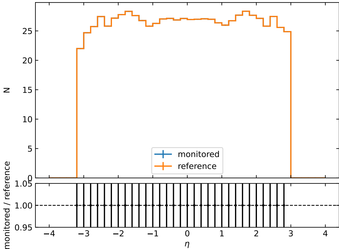
Number of total states vs. \eta
