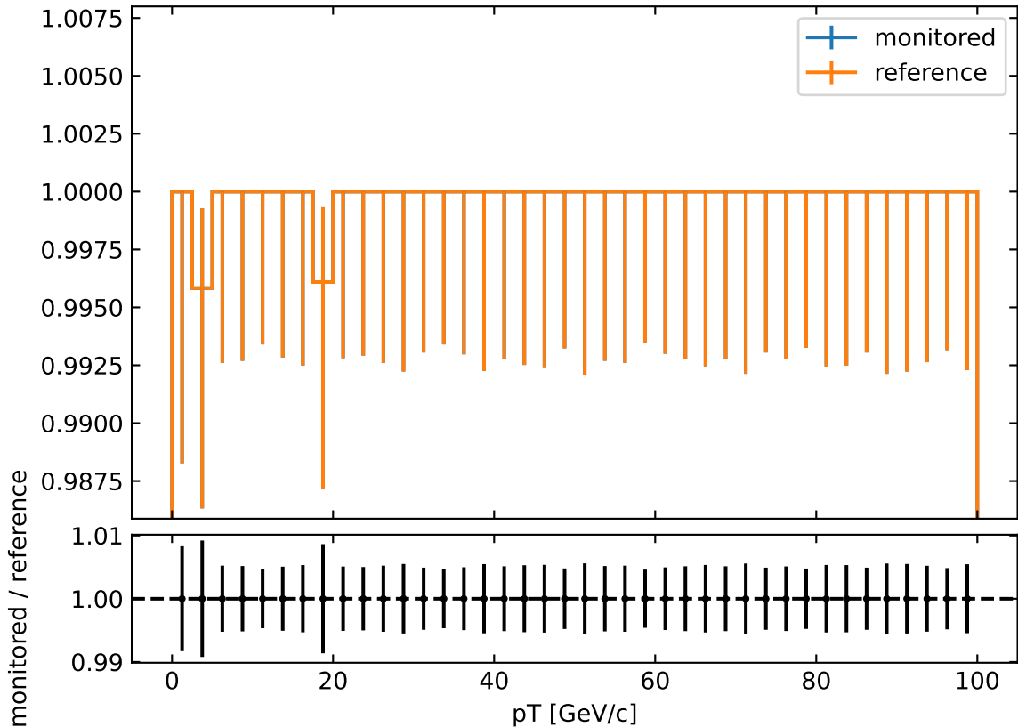
Tracking efficiency
