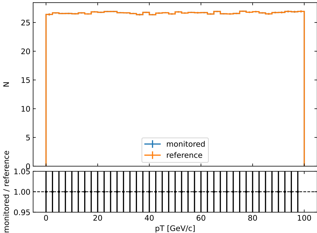
Number of total states vs. pT
