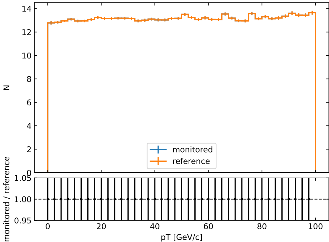
Number of measurements vs. pT
