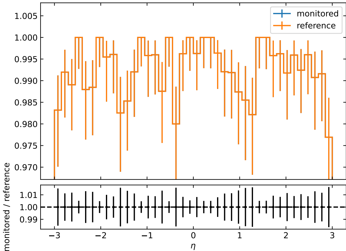
Tracking efficiency with p_T > 1 GeV/c
