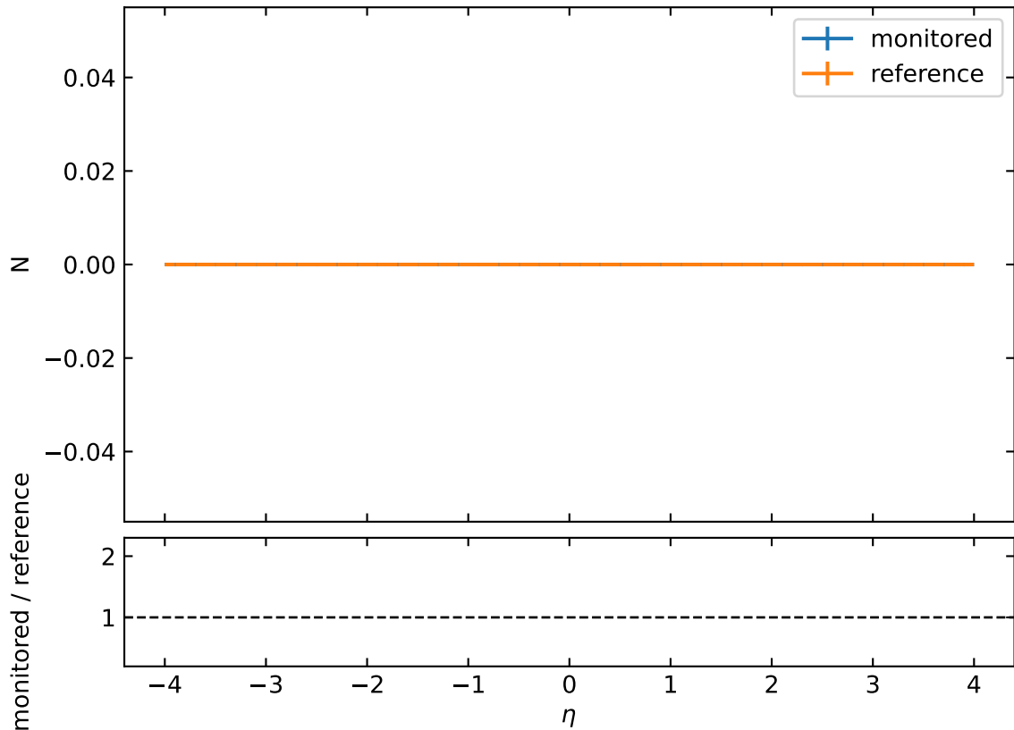
Number of Shared Hits vs. \eta
