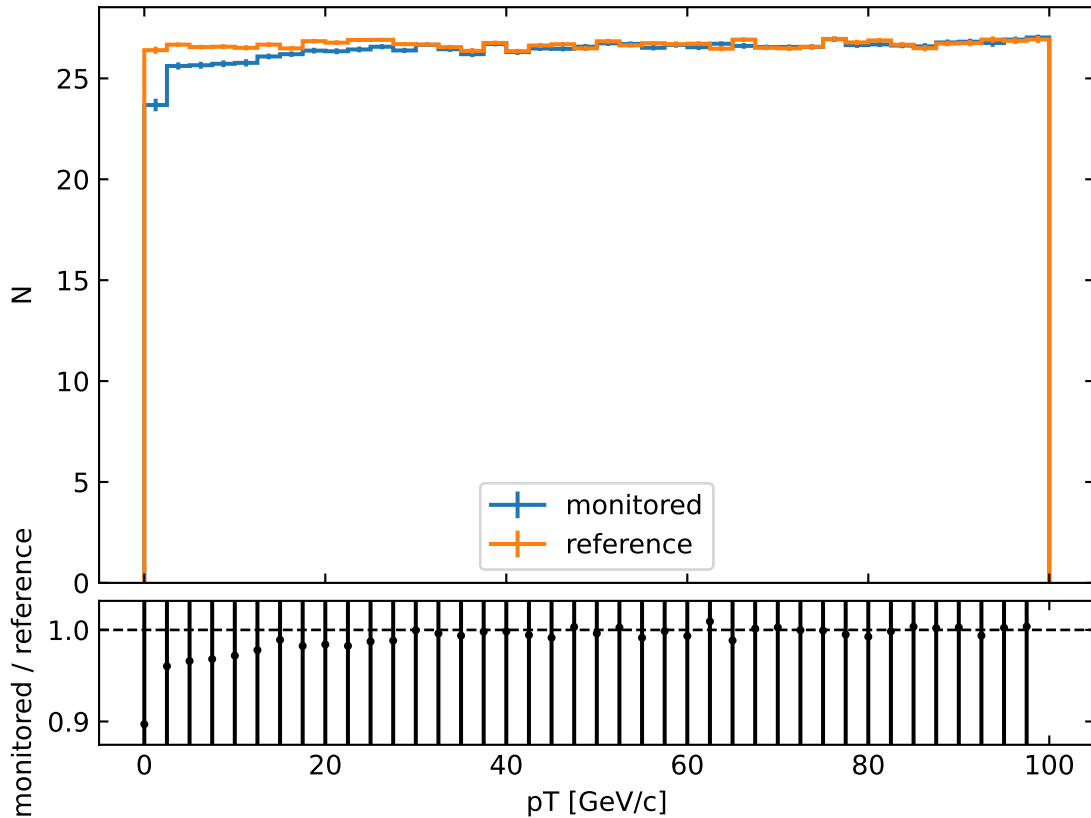
Number of total states vs. pT
