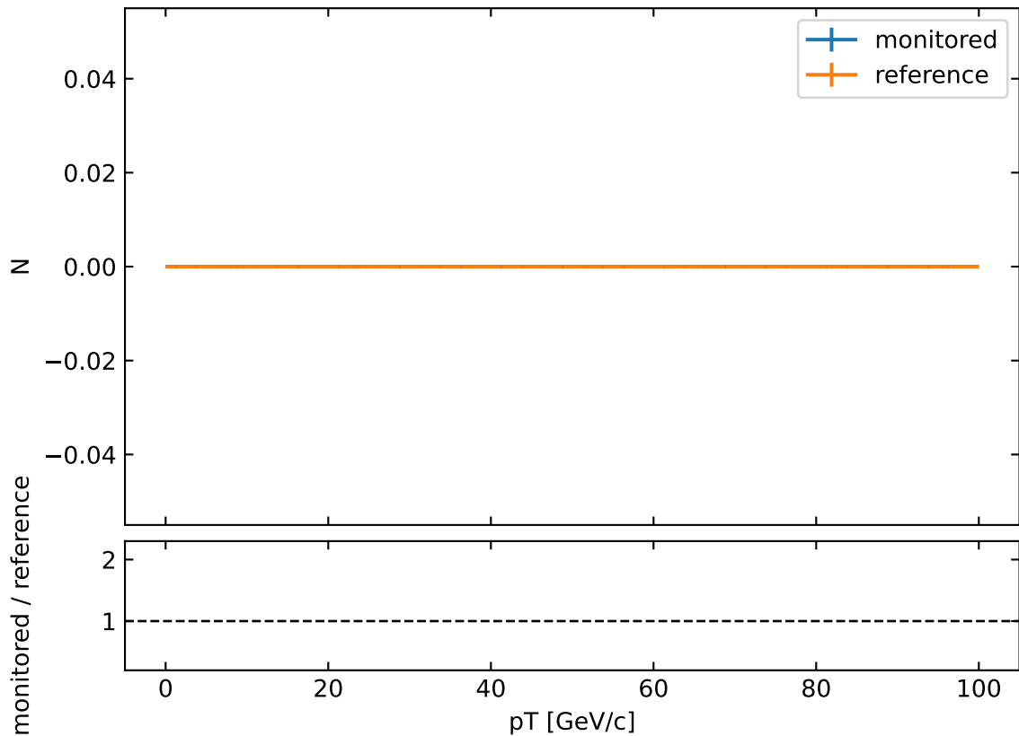
Number of Shared Hits vs. pT
