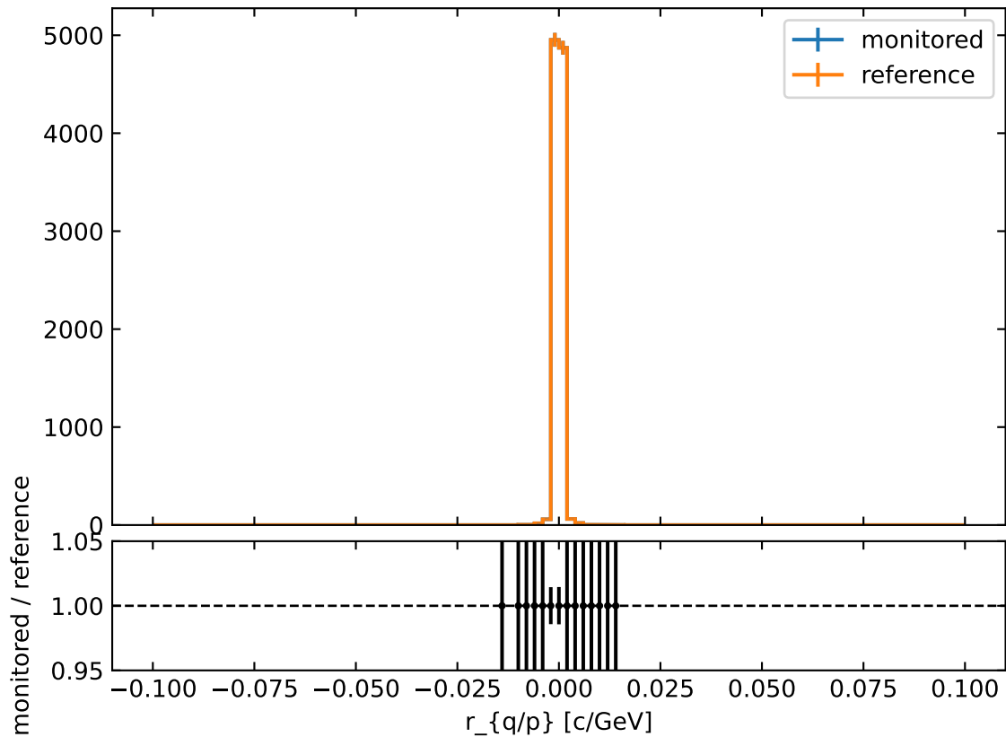
Residual of qop
