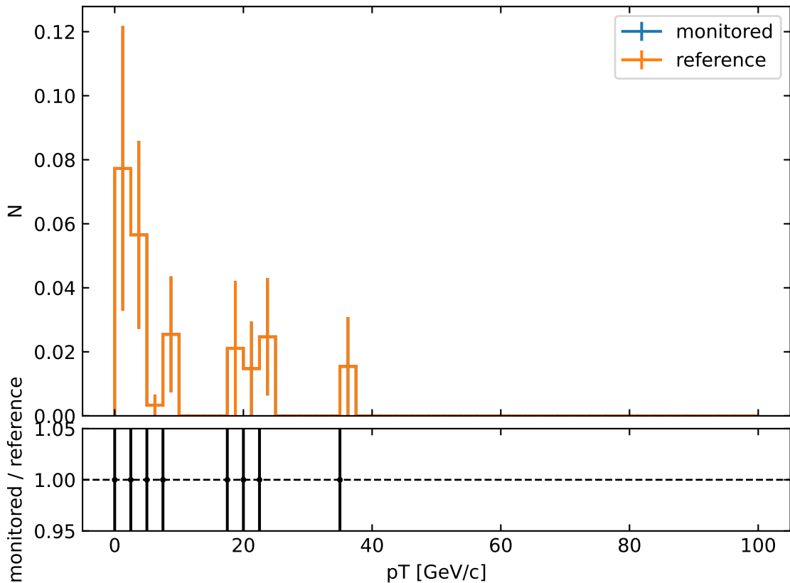
Number of outliers vs. pT
