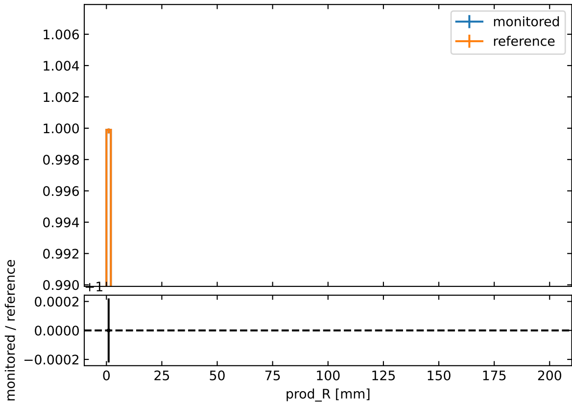
Tracking efficiency with p_T > 1 GeV/c
